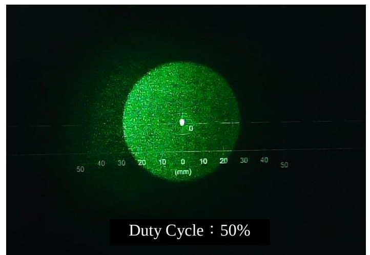
LM9G520H30P2T Beam Shape at 50cm
